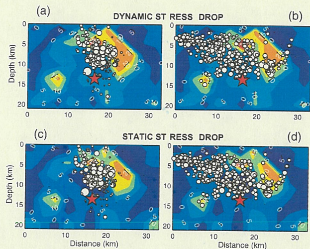
Figure 5. Comparison of the swarm seismic activity in 1989, 1990, 1997 (foreshocks) and aftershocks with the dynamic and static stress drop distribution; (a) foreshocks and dynamic stress drop; (b) aftershocks and dynamic stress drop; (c) foreshocks and static stress drop; (d) aftershocks and static stress drop.
